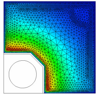
Square-LED: unstructured 3D grid with 85 000 cells
